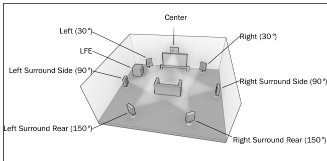
Configuration 2 - 7.1 channel: L, C, R, LFE, Ls, Rs, Lhs, Rhs
